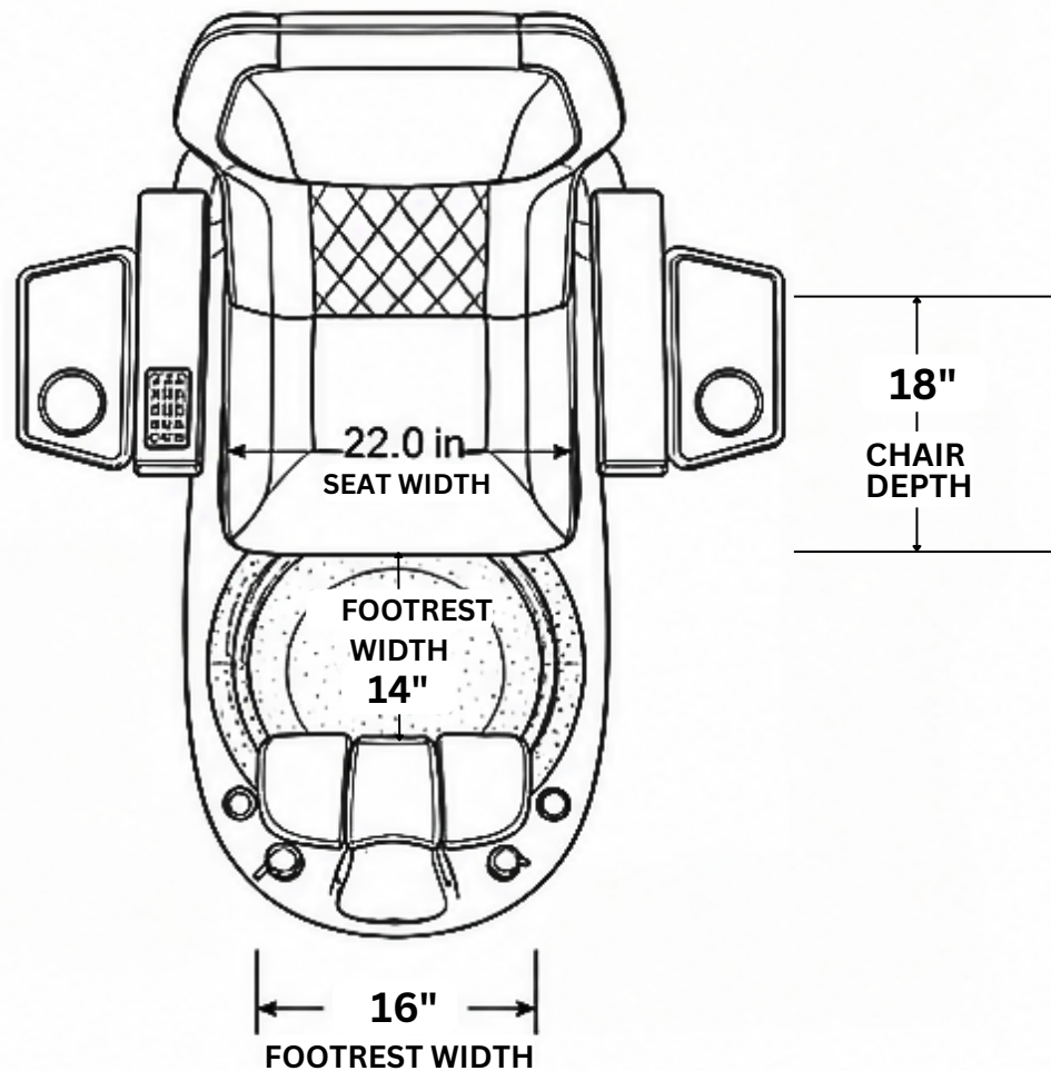
TOP VIEW
