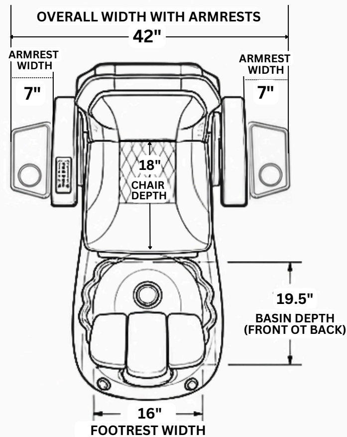
TOP VIEW
